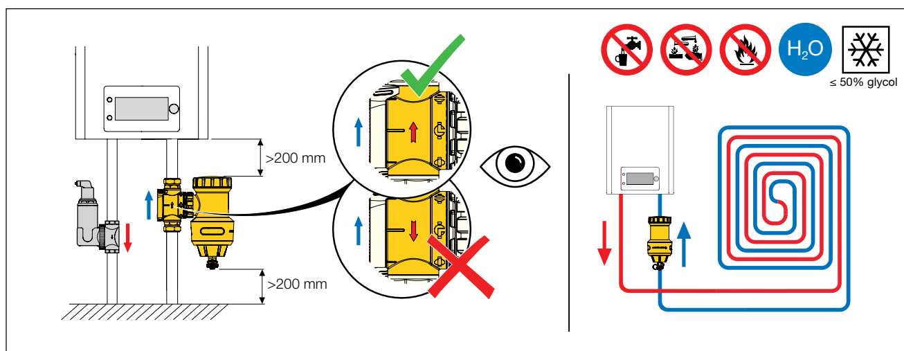
Figure 7: Positioning
