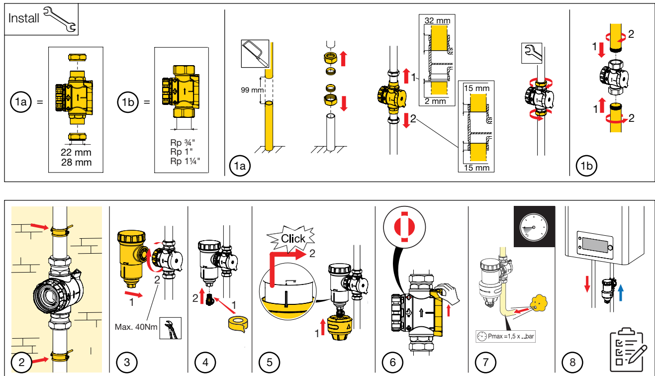
Figure 8: Installation
