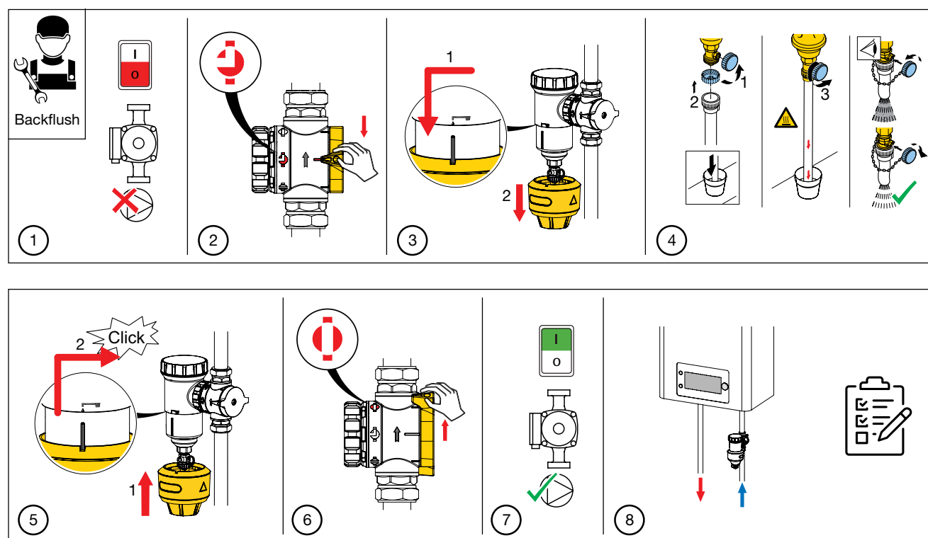
Figure 9: Backflush procedure
