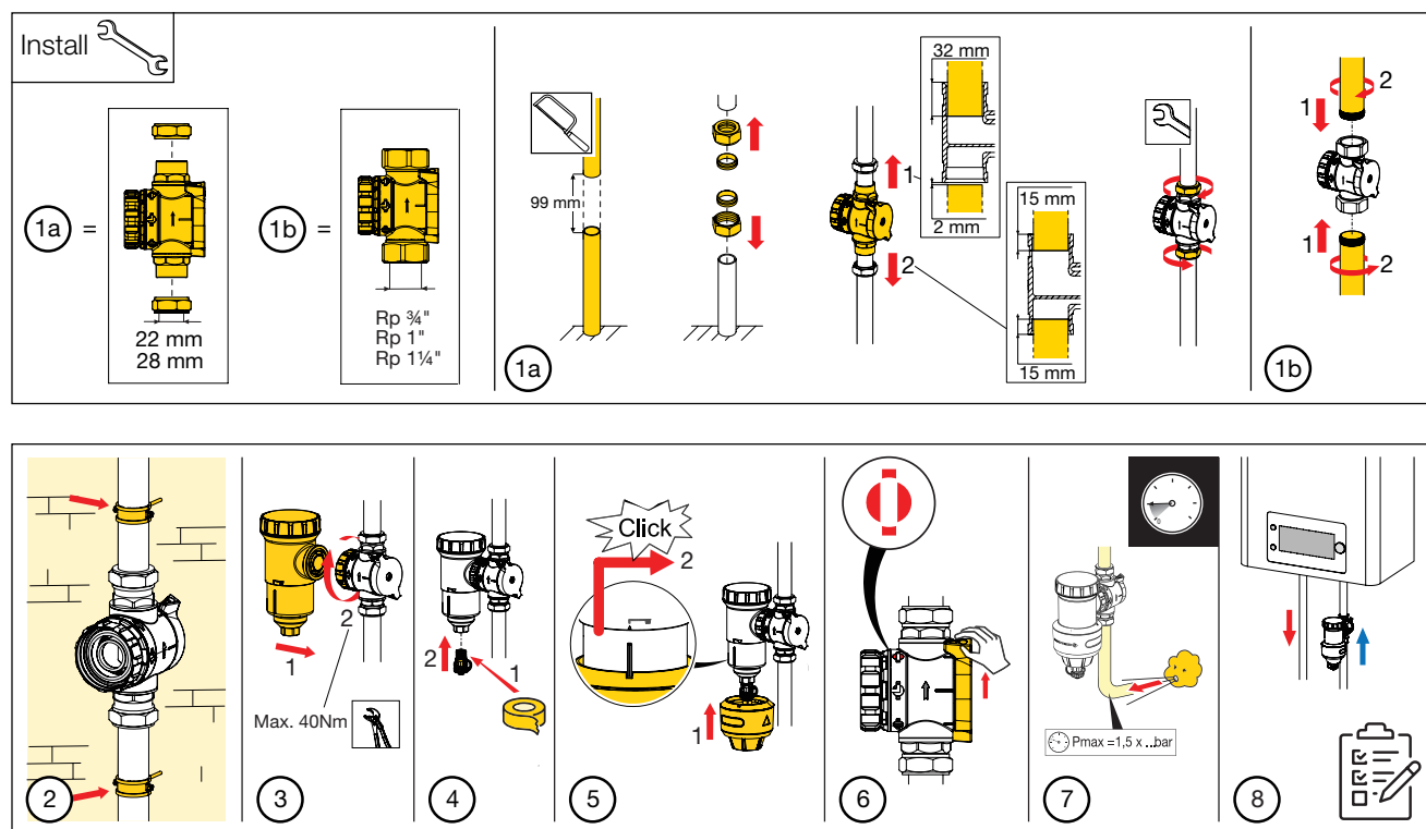
Figure 8: Installation
